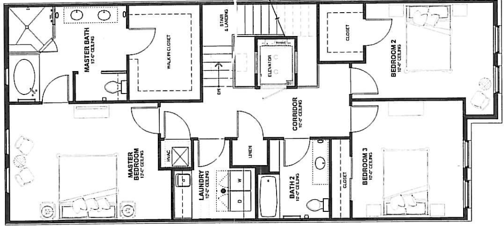
DUNBAR - 2A SECOND FLOOR PLAN Scale: 3/32" = 1'-0" 0 4' 8"
