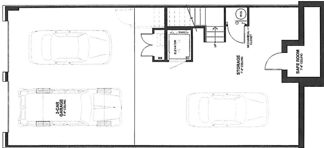
DUNBAR - 2A FIRST FLOOR PLAN Scale: 3/32" = 1'-0" 0 4' 8"
